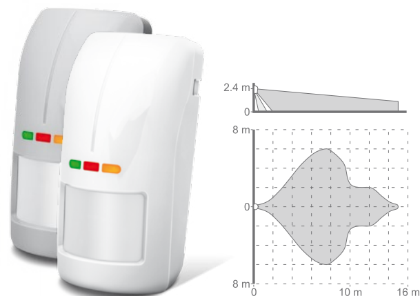
OPAL / OPAL GY / OPAL Plus / OPAL Plus GY
